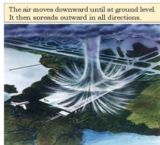
Figure 37 - Microburst
