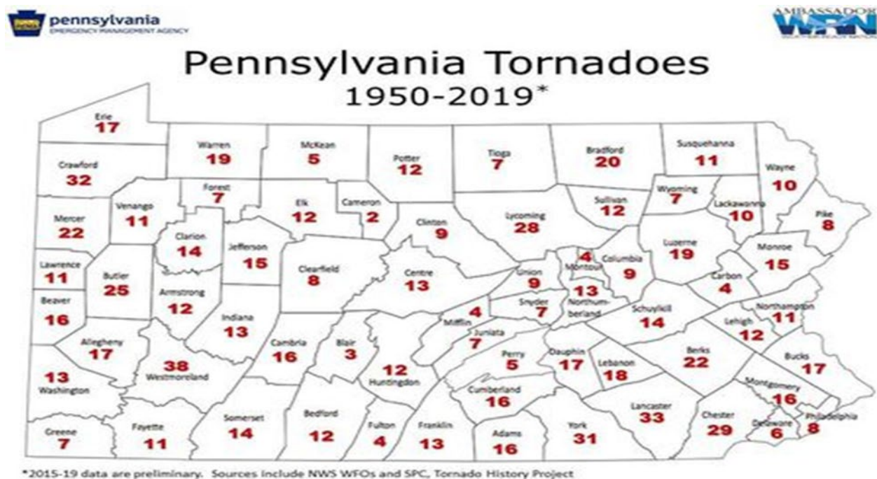
Figure 39 - Pennsylvania Tornadoes 1950-2019
